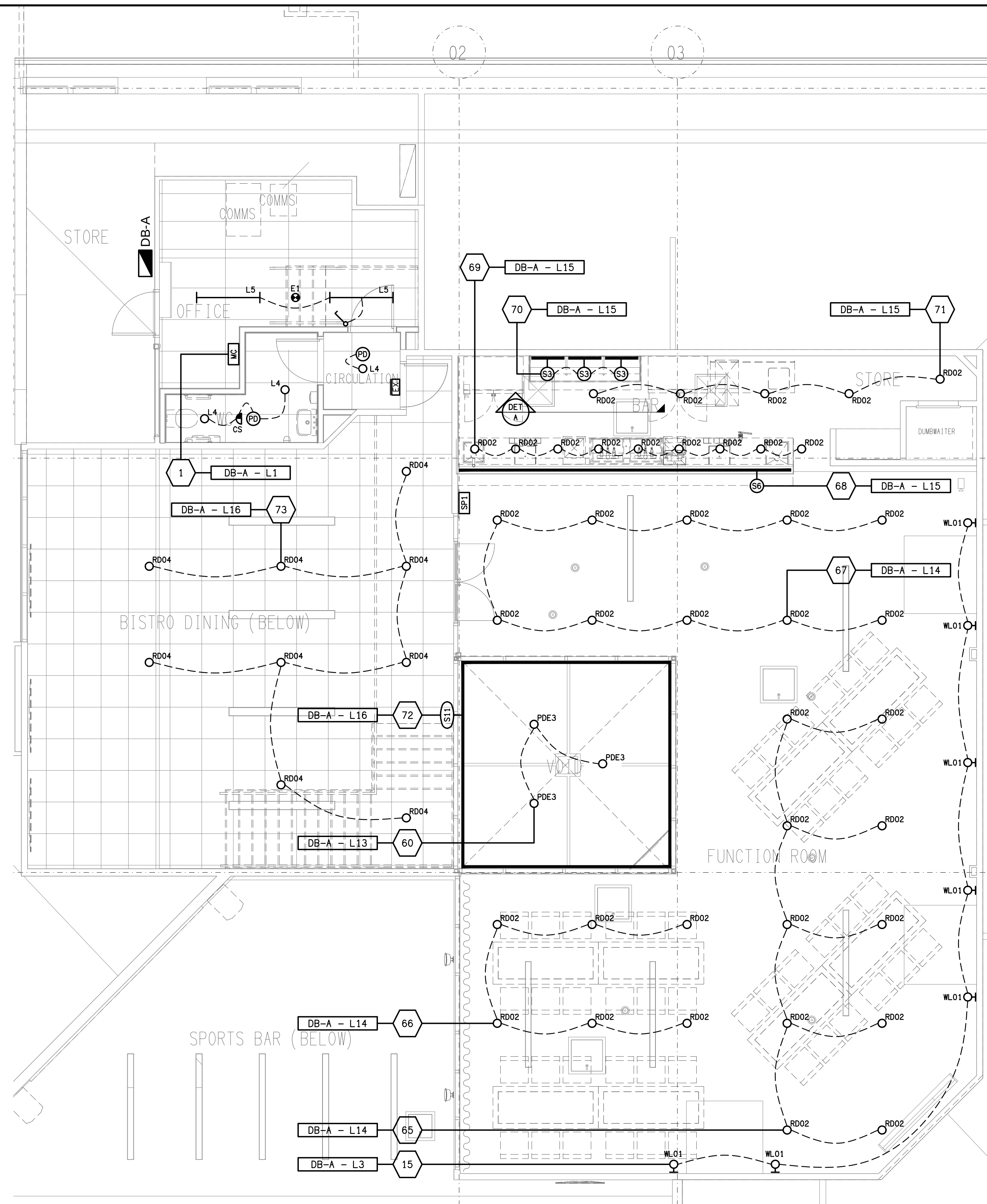
REFLECTED CEILING PLAN LEVEL 1 SCALE 1:50
