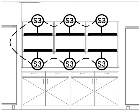
DETAIL A LEVEL 1 BAR ELEVATION SCALE 1: 50
